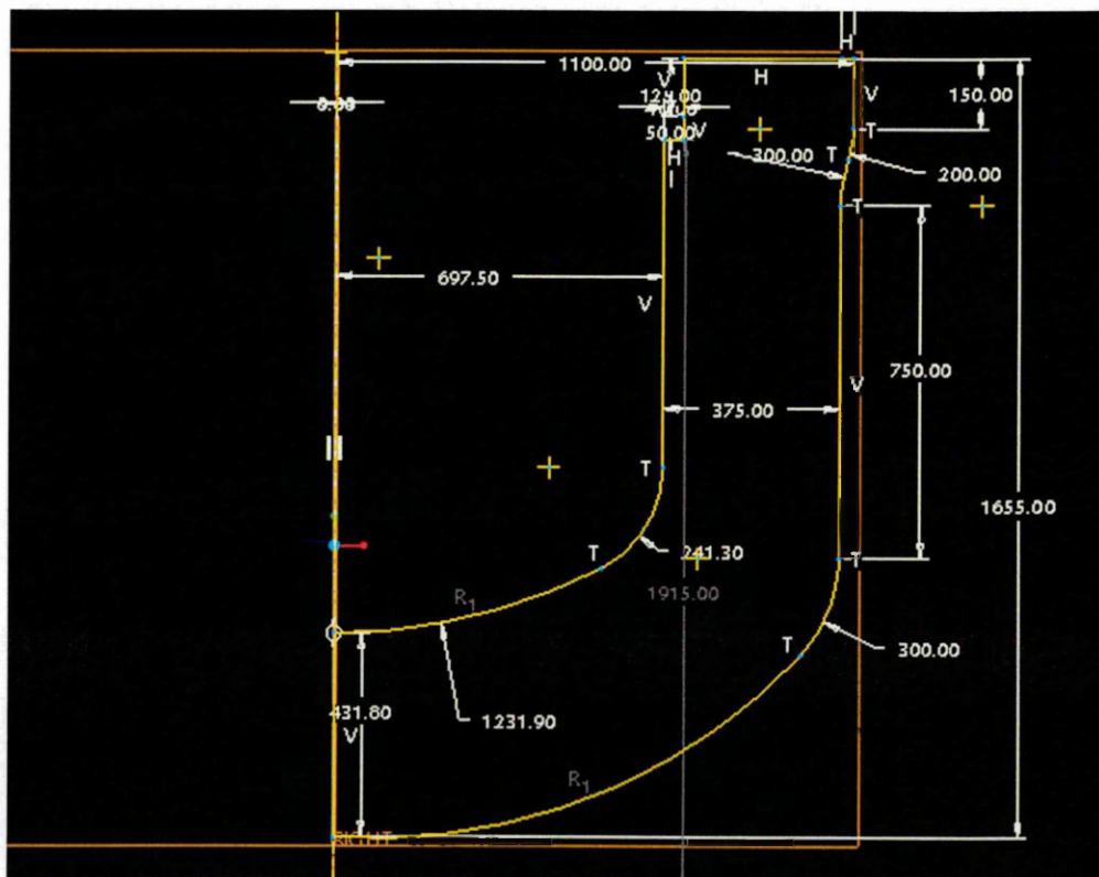
Figure 21: Cylinder Dimensions
