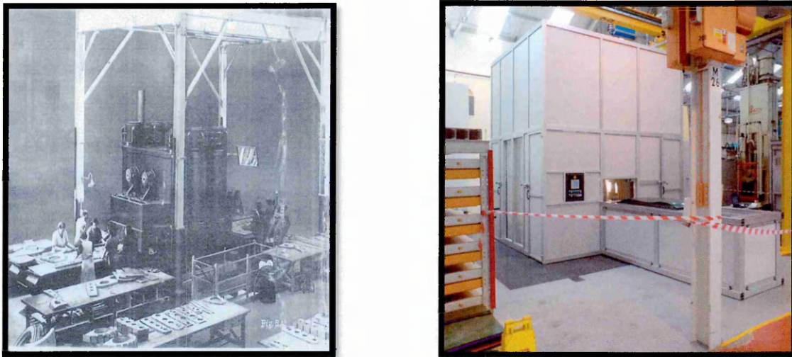
Figure 9: Rubber Die Press (1965 and 2008) - John Shaw and Joseph Rhodes Limited
