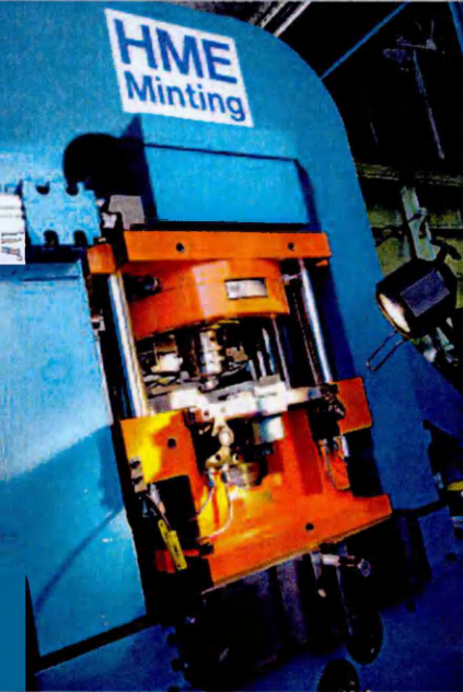
re: Front view of the optional HME fast Hydraulic Clamping System.
