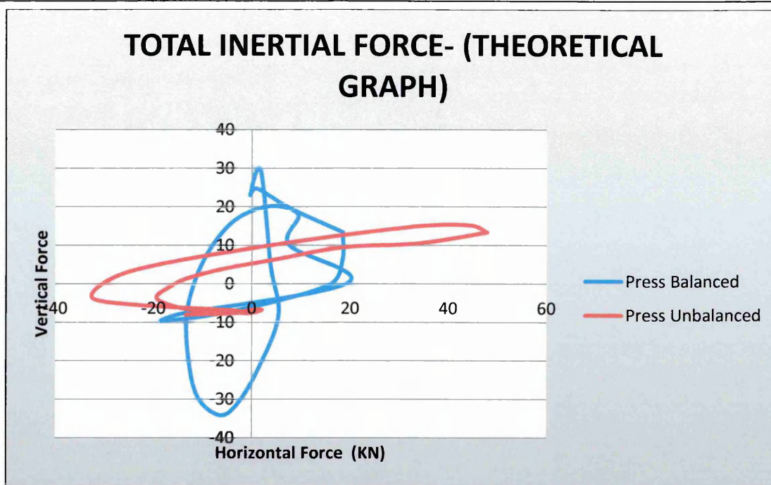
Figure 64: KJ Balancing - Total Inertial Force (Theoretical)
