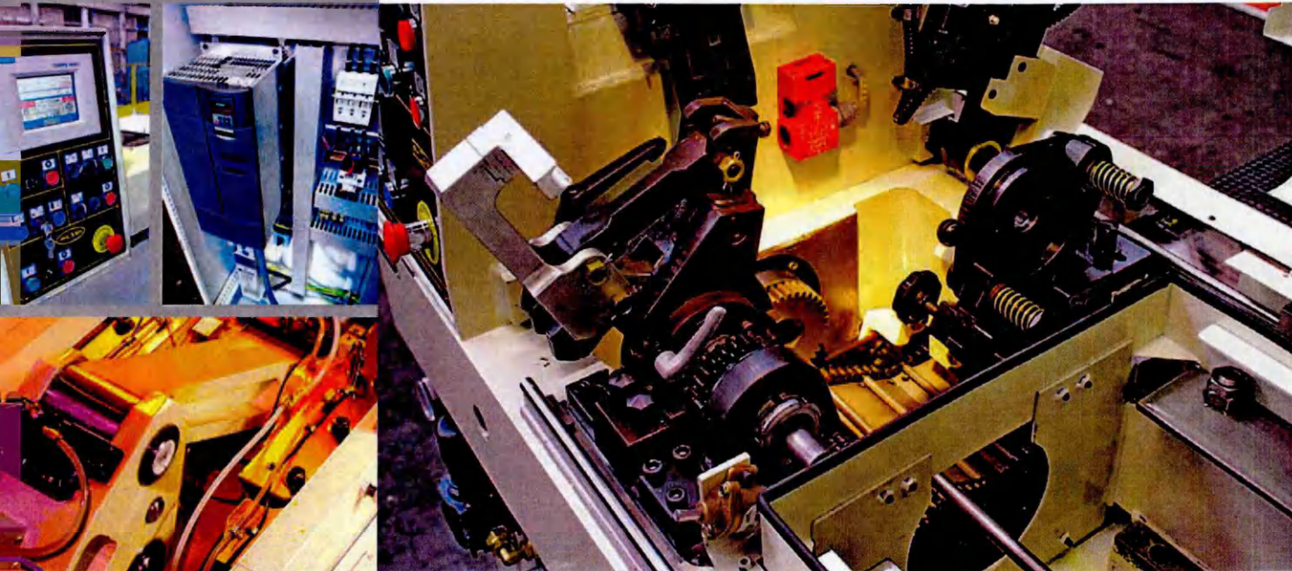
In (right): Tool space area showing feed plate, upper bracket and take-off system. (left): Integrated PLC touch screen control. (Also available as a free standing control unit). (right): AC main drive motor control. Bottom: KJX linkage system. Bottom: Slug feed arrangement.
