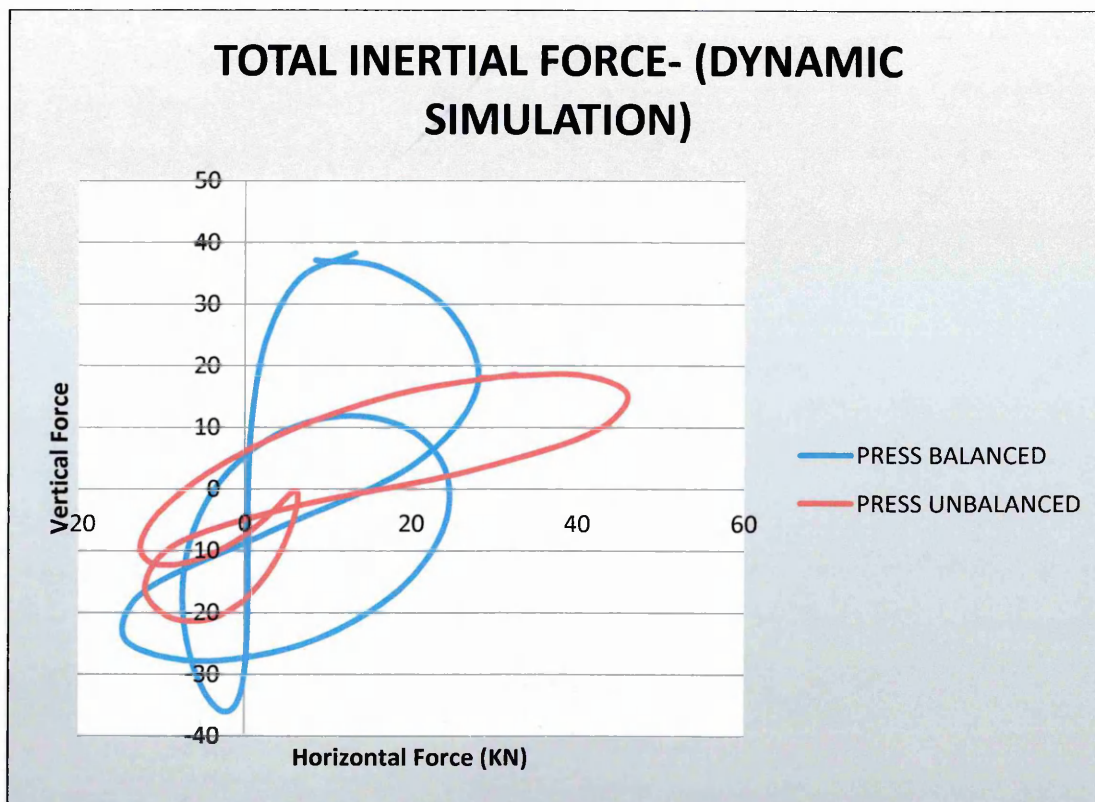
Figure 65: KJ Balancing - Total Inertial Force (Dynamic Simulation)
