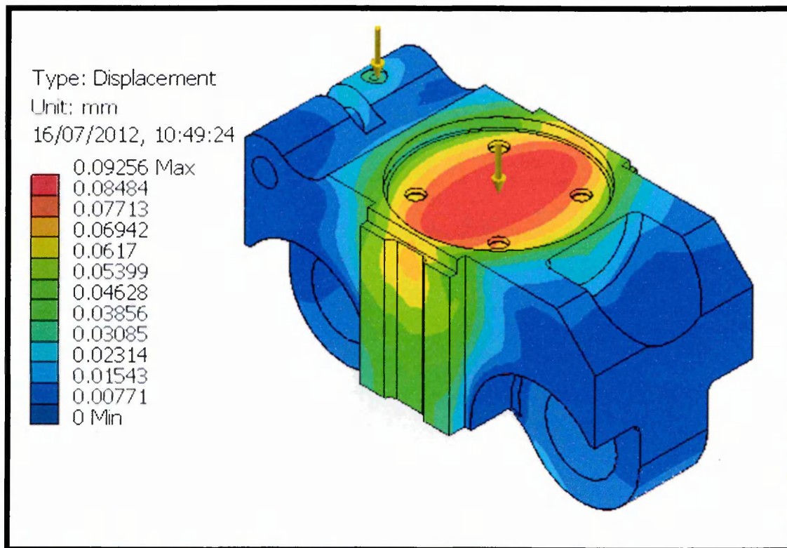
Figure 72: Displacement
