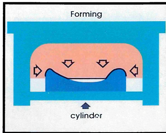
Figure 14: Principle of Operation - Forming
