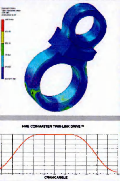
(Right): Tool area of press showing tooling dies and in situ. (Top): Stress analysis of upper link. (Bottom): Slide displacement graph showing dwell side dwell for reliable coin blank feeding and discharge.
