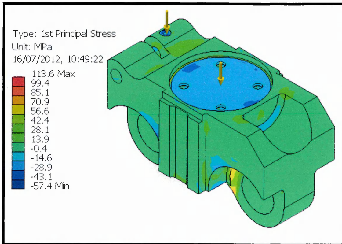
Figure 70: 1st Principal Stress
