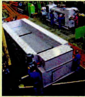
A Box Feeder and Centex 430 Extruder being assembled at the Wakefield site.
